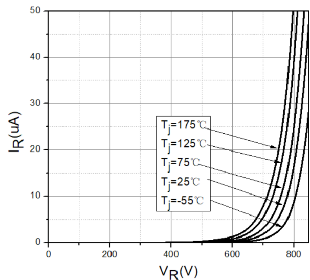
Figure2. Reverse Characteristic
