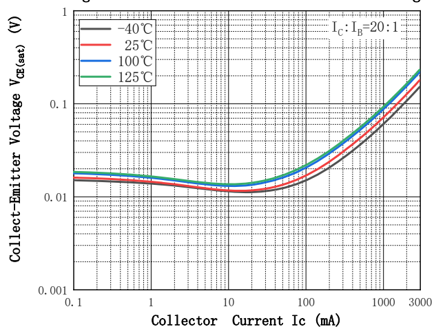
Fig.4 - Collect-Emittor Saturation Voltage
