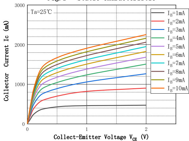
Fig.1 - Static characteristic
