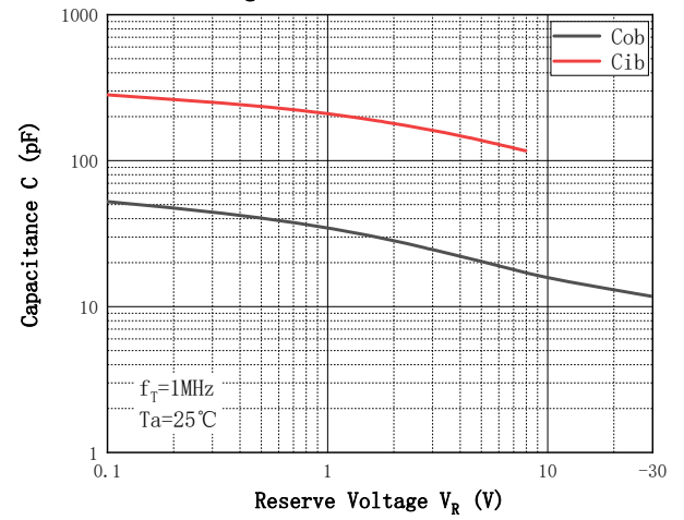
Fig.8 - Cob/Cib—VCB/VEB
