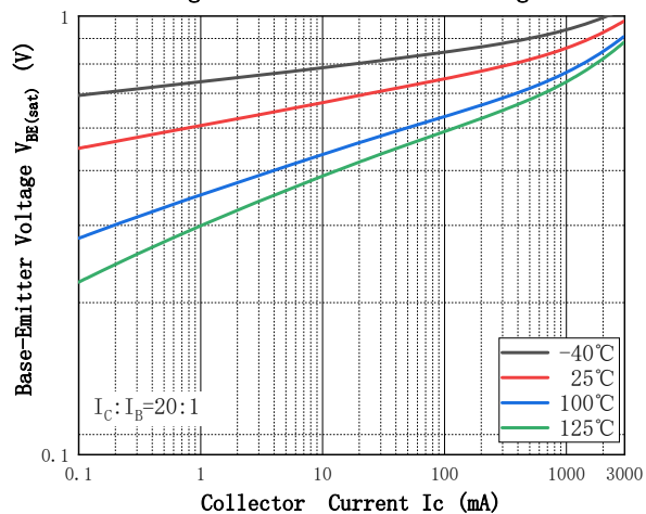
Fig.6 - Base-Emittor Voltage
