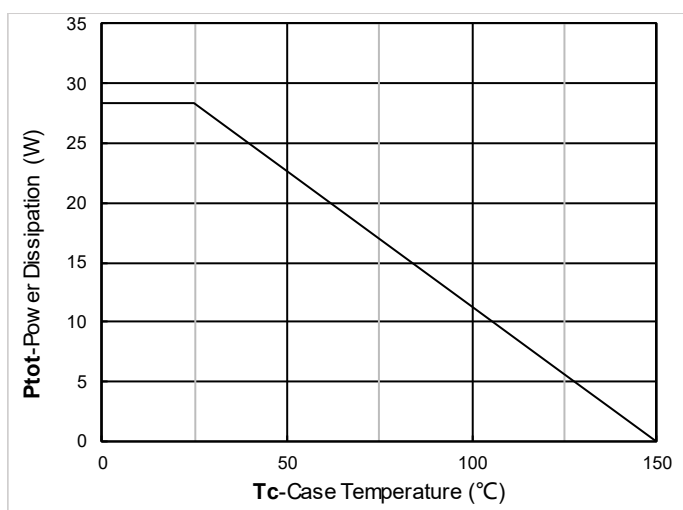
Figure 12. Power dissipation
