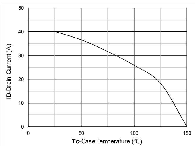
Figure 11. Current dissipation
